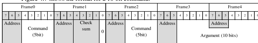
Figure 4.7 Data format of 10-bit command
