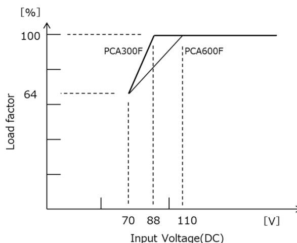
Figure 6.5.7 Input voltage derating curve (DC)
